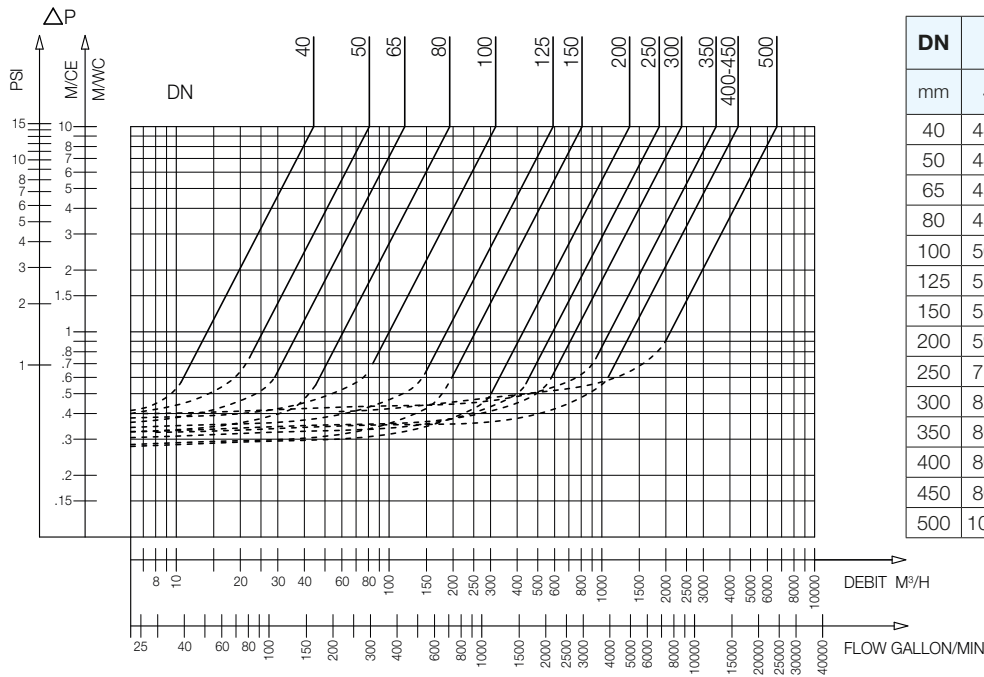
402 S - Headloss chart
